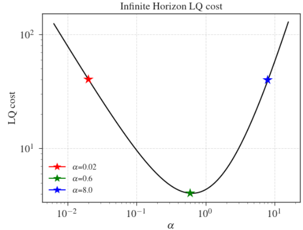
Fig. 1: Optimal infinite time LQ state feedback cost as a function of \alpha . Choices of 3 \alpha values for detailed study are highlighted. These values differ by 400x in \alpha and by 10x in cost.
